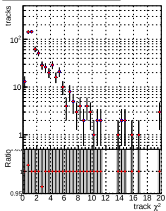
N of reco track vs. \chi^2 for DQM_CKF_TTbase (blue) and DQM_CKF_TT_retrainOldFiles125_v2_prelimWPM_epoch3 (red)
