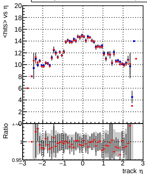
mean hits vs \eta Legend: DQM_CKF_TTbase (blue line), DQM_CKF_TT_retrainOldFiles125_v2_prelimWPM_epoch3 (red line)
