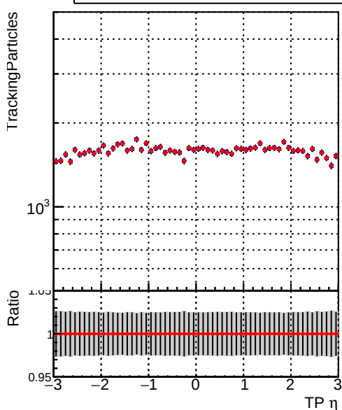
N of simulated tracks vs \eta Legend: - DQM_CKF_TTbase (blue squares) - DQM_CKF_TT_retrainOldFiles125_v2_prelimWPM_epoch2 (red circles)
