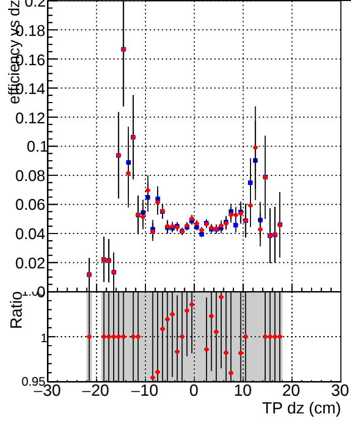
Efficiency vs Dz Legend: DQM_CKF_TTbase (Blue square) DQM_CKF_TT_retrainOldFiles125_v2_prelimWPM_epoch2 (Red circle)
