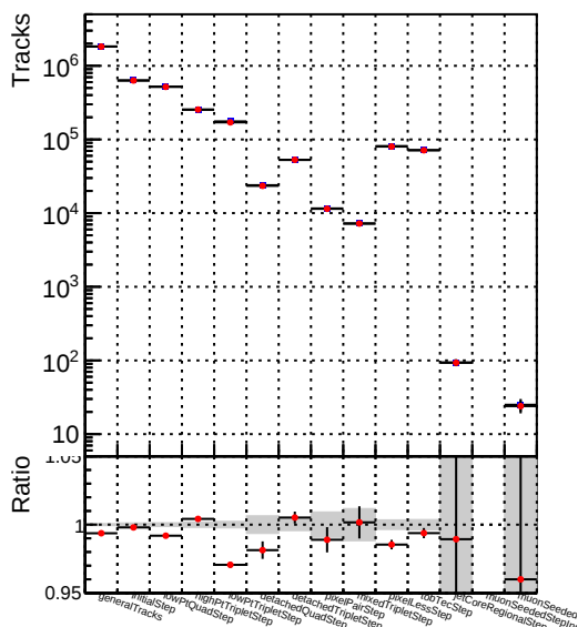
Number of tracks vs collection Legend: DQM_CKF_TTbase (blue line with circles), DQM_CKF_TT_retrainOldFiles125_v2_prelimWPM_epoch2 (red line with circles)
