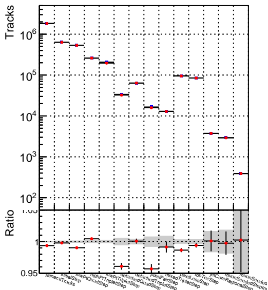
Legend: DQM_CKF_TTbase (blue square), DQM_CKF_TT_retrainOldFiles125_v2_prelimWPM_epoch2 (red circle)
