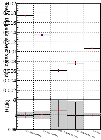
—•— DQM_CKF_TTbase —•— DQM_CKF_TT_retrainOldFiles125_v2_prelimWPM_epoch2
