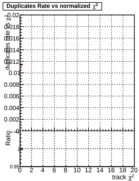
—•— DQM_CKF_TTbase —•— DQM_CKF_TT_retrainOldFiles125_v2_prelimWPM_epoch2
