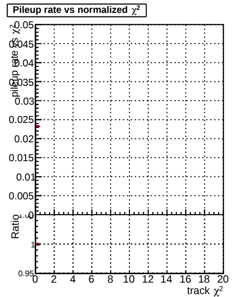
—•— DQM_CKF_TTbase —•— DQM_CKF_TT_retrainOldFiles125_v2_prelimWPM_epoch2
