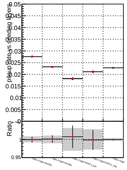
—•— DQM_CKF_TTbase —•— DQM_CKF_TT_retrainOldFiles125_v2_prelimWPM_epoch2
