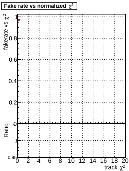
—•— DQM_CKF_TTbase —•— DQM_CKF_TT_retrainOldFiles125_v2_prelimWPM_epoch2
