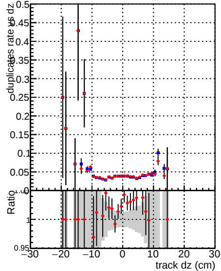
—●— DQM_CKF_TTbase —●— DQM_CKF_TT_retrainOldFiles125_v2_prelimWPM_epoch2
