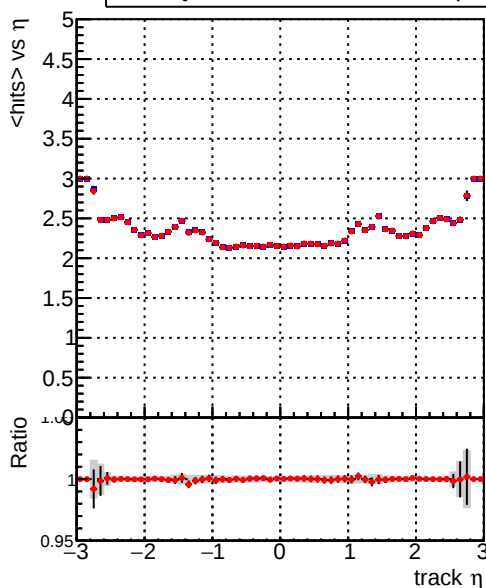
mean hits vs \eta Legend: DQM_CKF_TTbase (blue line), DQM_CKF_TT_retrainOldFiles125_v2_prelimWPM_epoch2 (red line)
