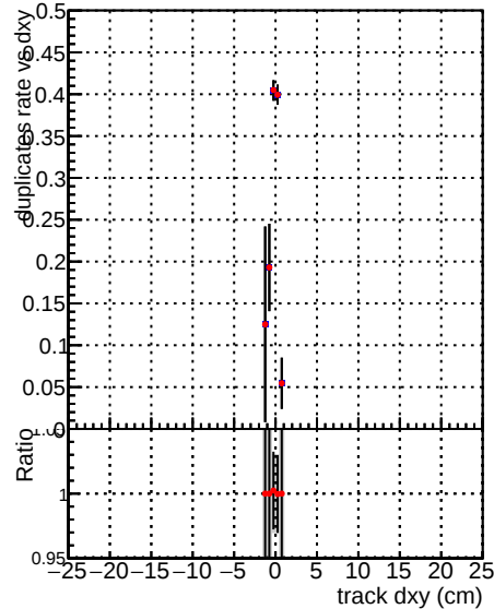
—●— DQM_CKF_TTbase —●— DQM_CKF_TT_retrainOldFiles125_v2_prelimWPM_epoch2
