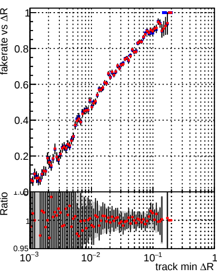
Legend: DQM_CKF_TTbase (black line with blue markers), DQM_CKF_TT_retrainOldFiles125_v2_prelimWPM_epoch2 (red line with red markers)
