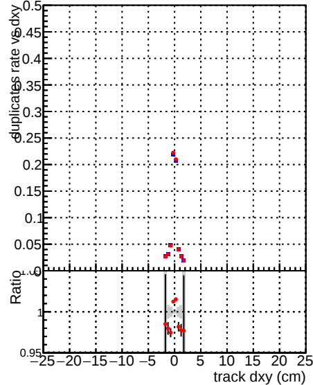
—●— DQM_CKF_TTbase —●— DQM_CKF_TT_retrainOldFiles125_v2_prelimWPM_epoch2
