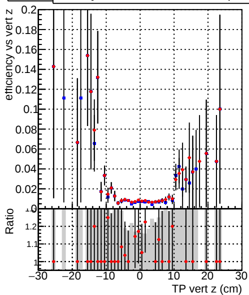
Efficiency vs vert z — DQM_CKF_TTbase — DQM_CKF_TT_retrainOldFiles125_v2_prelimWPM_epoch2
