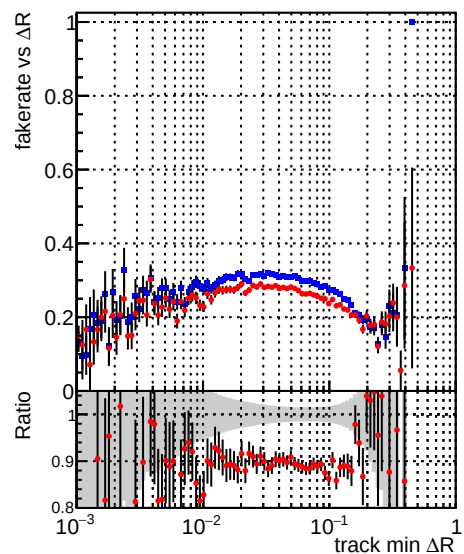
Legend: —•— DQM_CKF_TTbase —•— DQM_CKF_TT_retrainOldFiles125_v2_prelimWPM_epoch2
