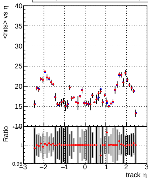
— DQM_CKF_TTbase — DQM_CKF_TT_retrainOldFiles125_v2_prelimWPM_epoch2
