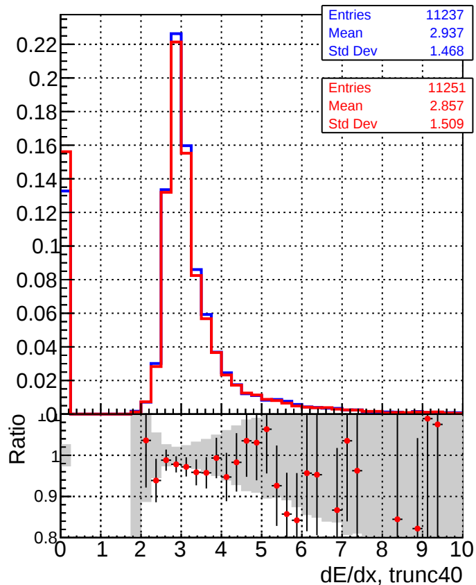
Legend: ■ DQM_CKF_TTbase ● DQM_CKF_TT_retrainOldFiles125_v2_prelimWPM_epoch2
