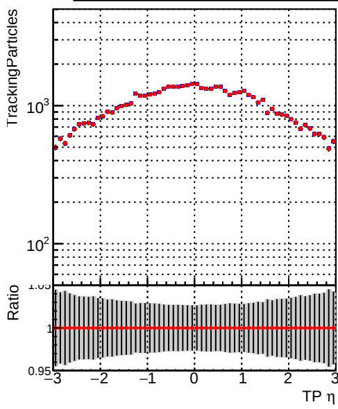
—•— DQM_CKF_TTbase —•— DQM_CKF_TT_retrainOldFiles125_v2_prelimWPM_epoch2
