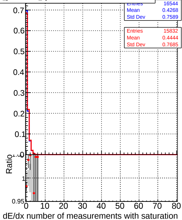
—■— DQM_CKF_TTbase —●— DQM_CKF_TT_retrainOldFiles125_v2_prelimWPM_epoch2
