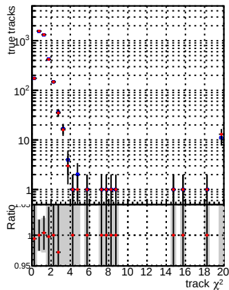
N of reco track vs. \chi^2 — DQM_CKF_TTbase — DQM_CKF_TT_retrainOldFiles125_v2_prelimWPM_epoch2
