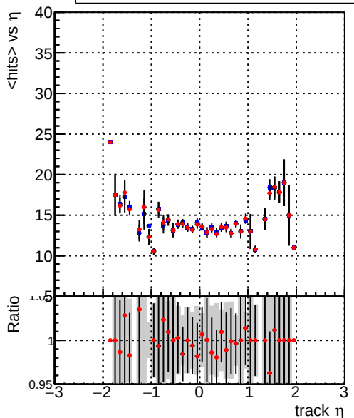
mean hits vs \eta — DQM_CKF_TTbase — DQM_CKF_TT_retrainOldFiles125_v2_prelimWPM_epoch2
