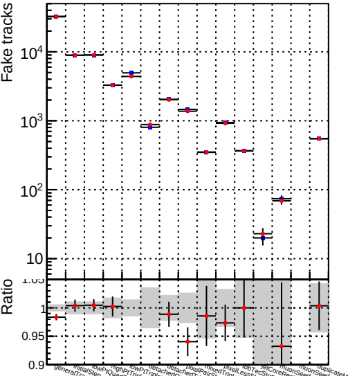
Number 1 DQM_CKF_TT_retrainOldFiles125_v2_prelimWPM_epoch2
