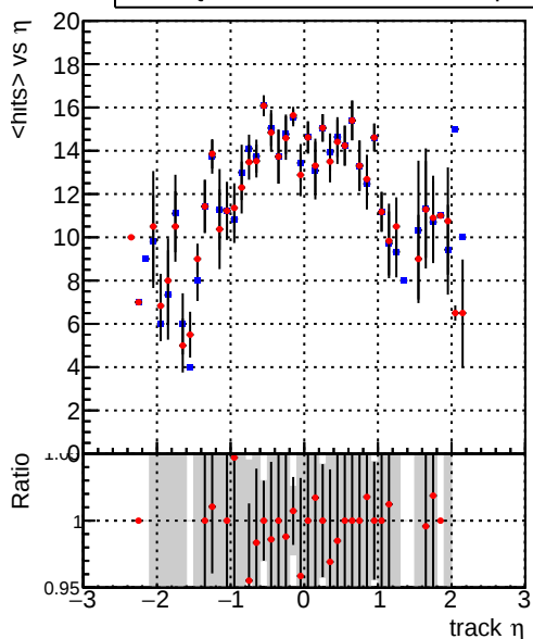
mean hits vs \eta Legend: DQM_CKF_TTbase (blue line with dots), DQM_CKF_TT_retrainOldFiles125_v2_prelimWPM_epoch2 (red line with dots)
