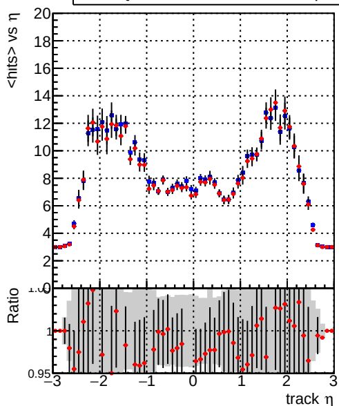
— DQM_CKF_TTbase — DQM_CKF_TT_retrainOldFiles125_v2_prelimWPM_epoch2
