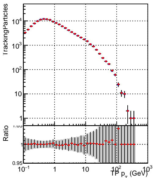
—•— DQM_CKF_TTbase —•— DQM_CKF_TT_retrainOldFiles125_v2_prelimWPM_epoch2
