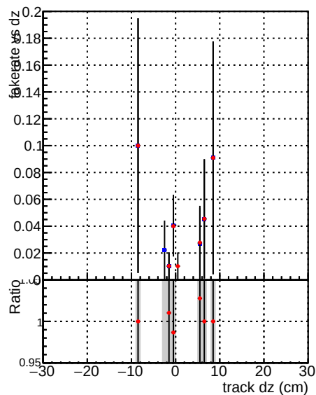
—•— DQM_CKF_TTbase —•— DQM_CKF_TT_retrainOldFiles125_v2_prelimWPM_epoch2
