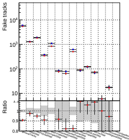
Number of tracks vs collection Legend: DQM_CKF_TTbase (blue line with dots), DQM_CKF_TT_retrainOldFiles125_v2_prelimWPM_epoch2 (red line with dots)
