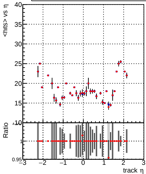
mean hit — DQM_CKF_TTbase — DQM_CKF_TT_retrainOldFiles125_v2_prelimWPM_epoch2
