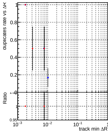
—●— DQM_CKF_TTbase —●— DQM_CKF_TT_retrainOldFiles125_v2_prelimWPM_epoch2
