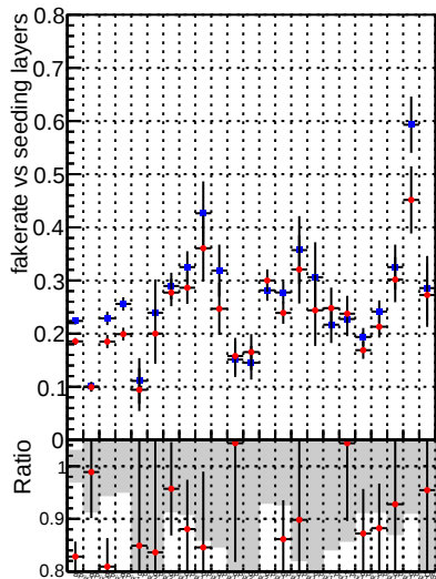
Fake rate vs. —•— DQM_CKF_TTbase —•— DQM_CKF_TT_retrainOldFiles125_v2_prelimWPM_epoch2
