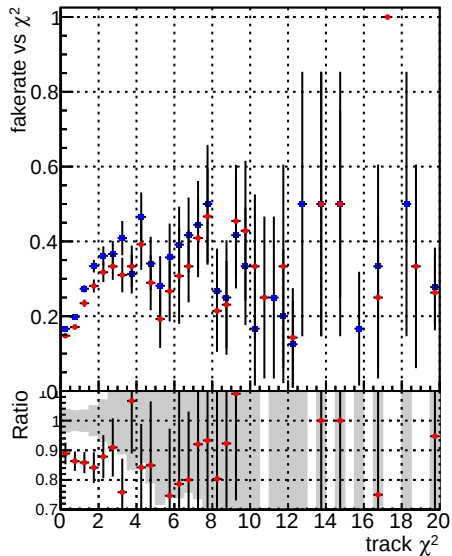
Fake rate vs. —•— DQM_CKF_TTbase —•— DQM_CKF_TT_retrainOldFiles125_v2_prelimWPM_epoch2
