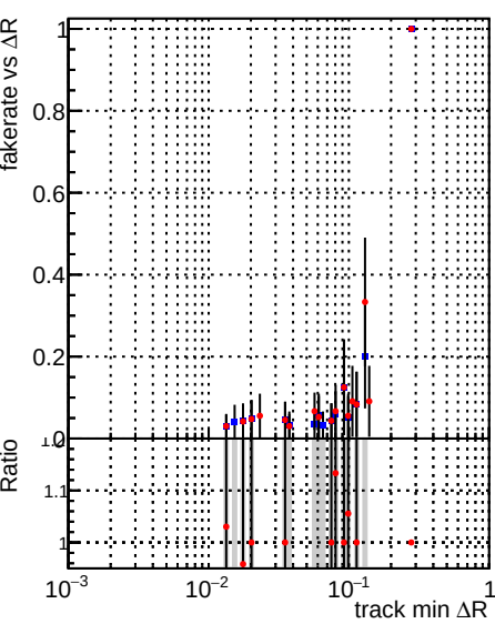
Legend: DQM_CKF_TTbase (blue squares), DQM_CKF_TT_retrainOldFiles125_v2_prelimWPM_epoch2 (red circles)
