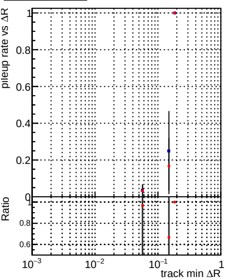
Legend: DQM_CKF_TTbase (blue squares), DQM_CKF_TT_retrainOldFiles125_v2_prelimWPM_epoch2 (red circles)
