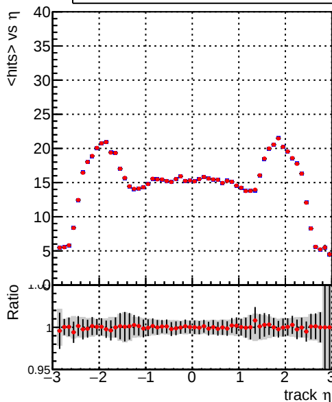
mean hits vs \eta Legend: DQM_CKF_TTbase (blue line with markers), DQM_CKF_TT_retrainOldFiles125_v2_prelimWPM_epoch2 (red line with markers)
