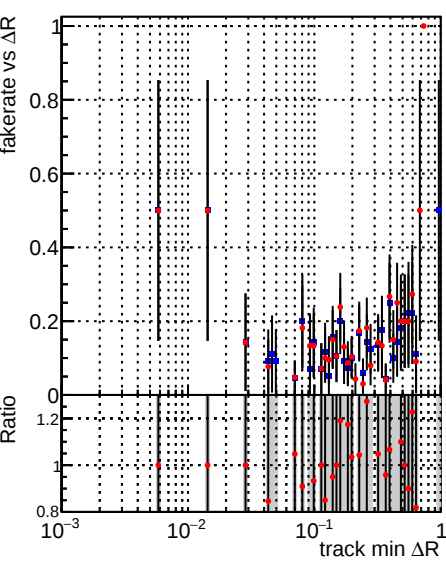
Legend: DQM_CKF_TTbase (blue stars), DQM_CKF_TT_retrainOldFiles125_v2_prelimWPM_epoch2 (red stars)
