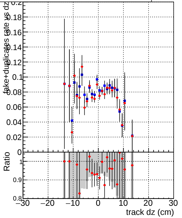
Legend: ■ DQM_CKF_TTbase ● DQM_CKF_TT_retrainOldFiles125_v2_prelimWPM_epoch2
