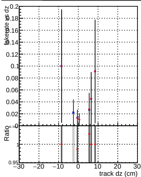
—●— DQM_CKF_TTbase —●— DQM_CKF_TT_retrainOldFiles125_v2_prelimWPM_epoch2
