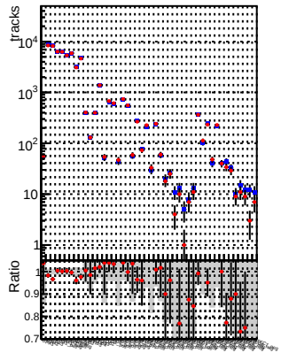
N of reco track vs. \chi^2 —●— DOM_CKF_TTbase —●— DOM_CKF_TT_retrainOldFiles125_v2_prelimWPM_epoch2
