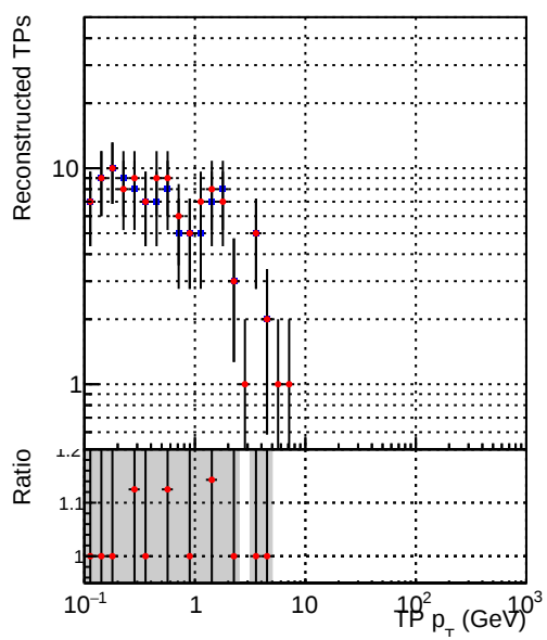
Legend: DQM_CKF_TTbase (blue square), DQM_CKF_TT_retrainOldFiles125_v2_prelimWPM_epoch2 (red circle)
