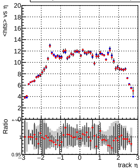
— DQM_CKF_TTbase — DQM_CKF_TT_retrainOldFiles125_v2_prelimWPM_epoch2 mean hits vs \eta
