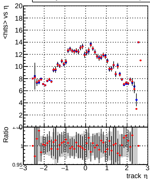
mean hits vs \eta Legend: DQM_CKF_TTbase (blue line with points), DQM_CKF_TT_retrainOldFiles125_v2_prelimWPM_epoch2 (red line with points)
