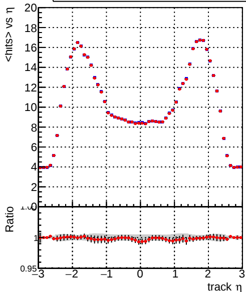
— DQM_CKF_TTbase — DQM_CKF_TT_retrainOldFiles125_v2_prelimWPM_epoch2
