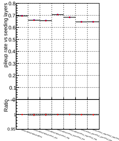
Pileup rate vs seeding layers
