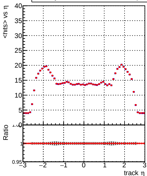
mean hits > \eta — DQM_CKF_TTbase — DQM_CKF_TT_retrainOldFiles125_v2_prelimWPM_epoch2
