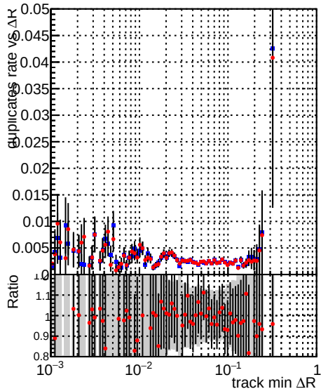
Legend: DQM_CKF_TTbase (blue line with error bars) DQM_CKF_TT_retrainOldFiles125_v2_prelimWPM_epoch2 (red line with error bars)
