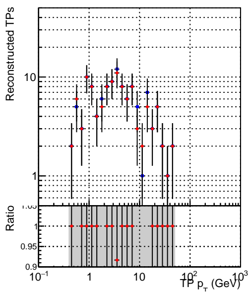
Legend: - DQM_CKF_TTbase (grey) - DQM_CKF_TT_retrainOldFiles125_v2_prelimWPM_epoch2 (red)
