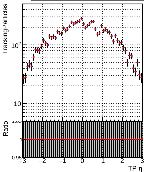
Legend: DQM_CKF_TTbase (blue line), DQM_CKF_TT_retrainOldFiles125_v2_prelimWPM_epoch2 (red line)
