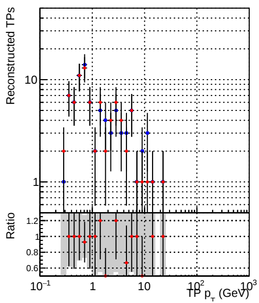
—•— DQM_CKF_TTbase —•— DQM_CKF_TT_retrainOldFiles125_v2_prelimWPM_epoch2
