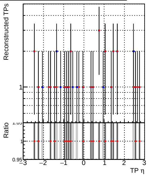
—•— DQM_CKF_TTbase —•— DQM_CKF_TT_retrainOldFiles125_v2_prelimWPM_epoch2
