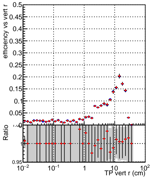
Legend for all plots: — DQM_CKF_TTbase (blue squares) — DQM_CKF_TT_retrainOldFiles125_v2_prelimWPM_epoch2 (red circles)
