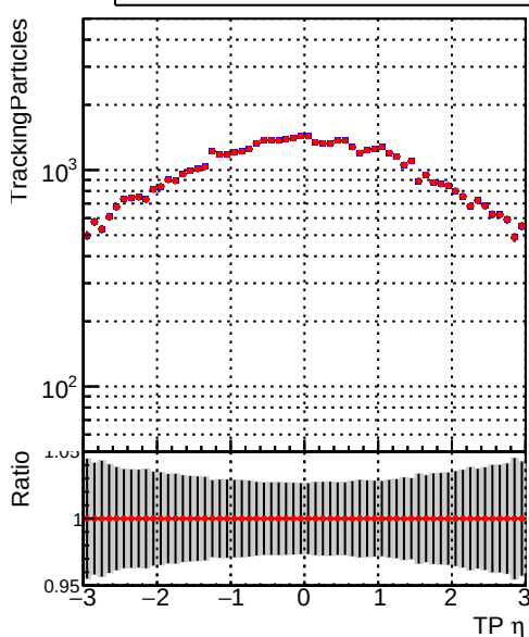
N of simulated tracks vs \eta Legend: \blacksquare DQM_CKF_TTbase \bullet DQM_CKF_TT_retrainOldFiles125_v2_prelimWPM_epoch2
