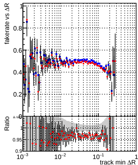
— DQM_CKF_TTbase — DQM_CKF_TT_retrainOldFiles125_v2_prelimWPM_epoch2
