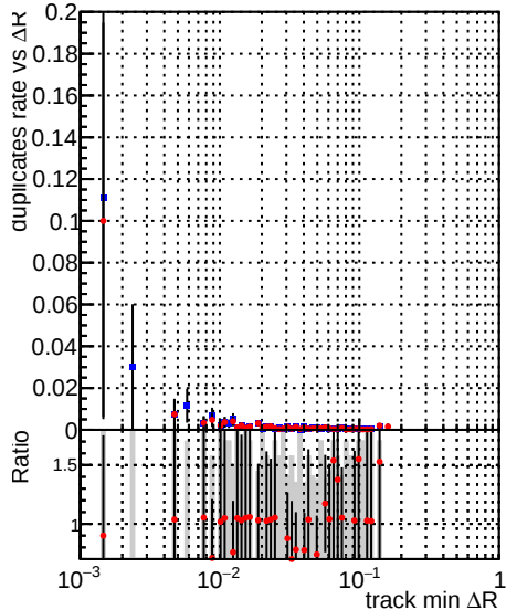
— DQM_CKF_TTbase — DQM_CKF_TT_retrainOldFiles125_v2_prelimWPM_epoch2
