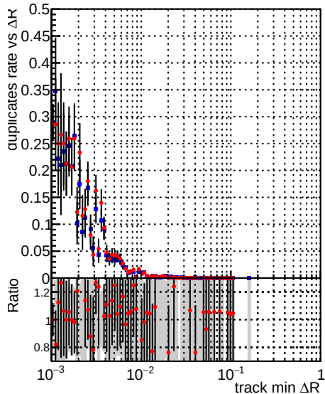
—•— DQM_CKF_TTbase —•— DQM_CKF_TT_retrainOldFiles125_v2_prelimWPM_epoch2
