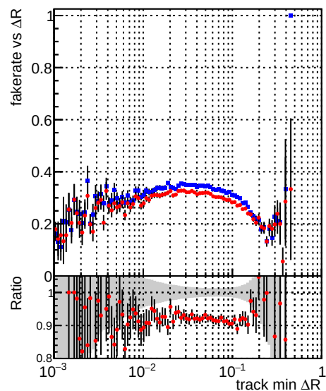
—•— DQM_CKF_TTbase —•— DQM_CKF_TT_retrainOldFiles125_v2_prelimWPM_epoch2
