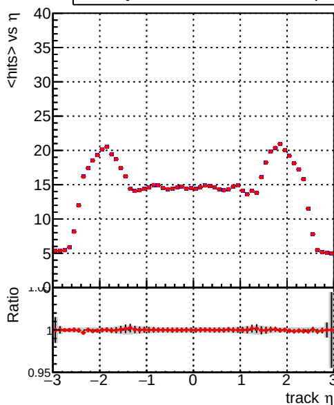
— DQM_CKF_TTbase — DQM_CKF_TT_retrainOldFiles125_v2_prelimWPM_epoch2
